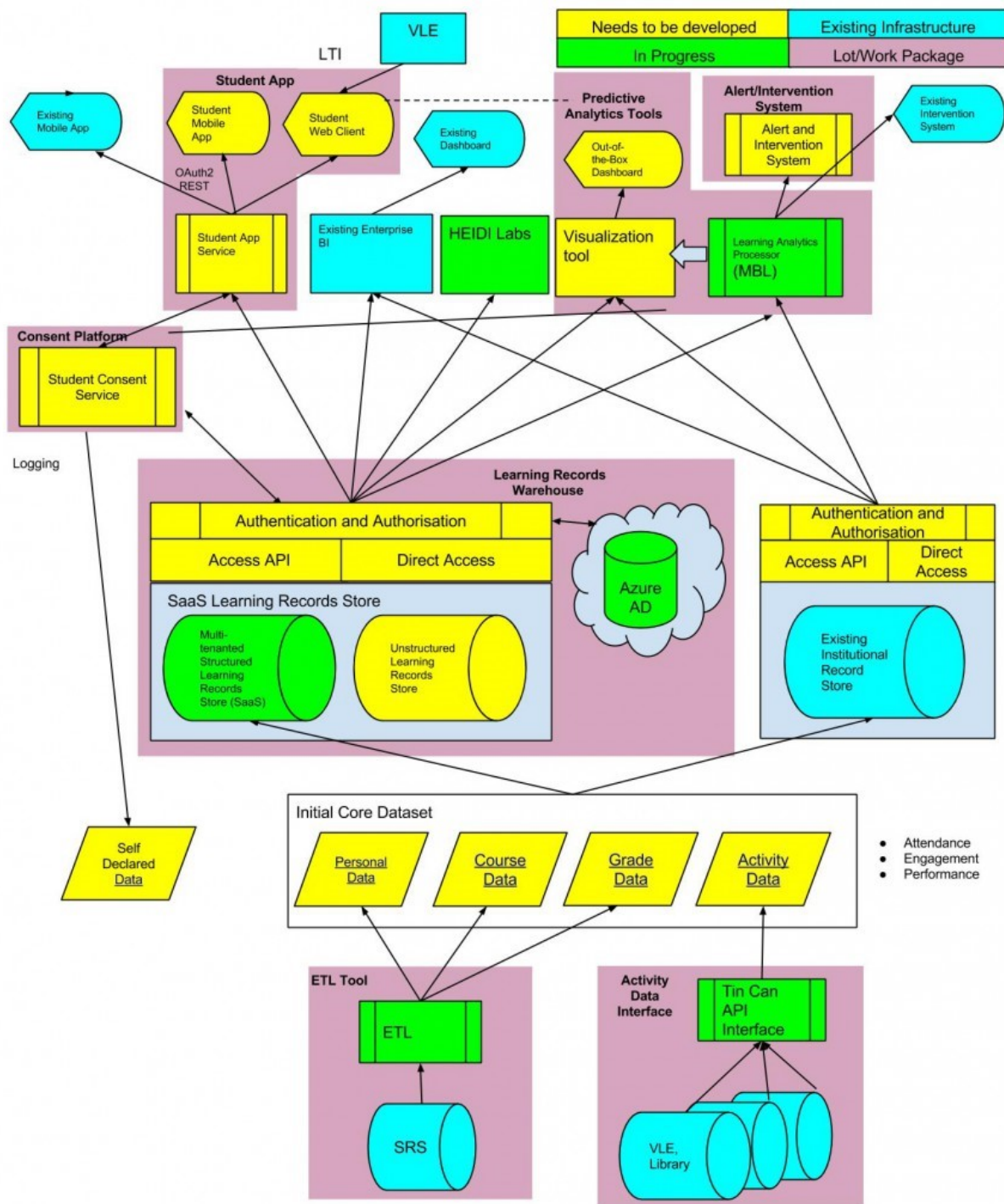
Figure 1: Jisc’s architecture for learning analytics
